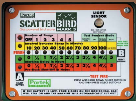
Simple push button controls
